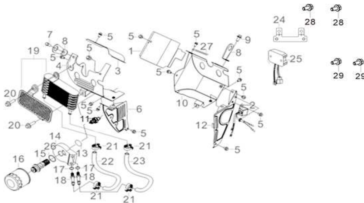
FIG.7 SHROUD/LOWER SHIELD
