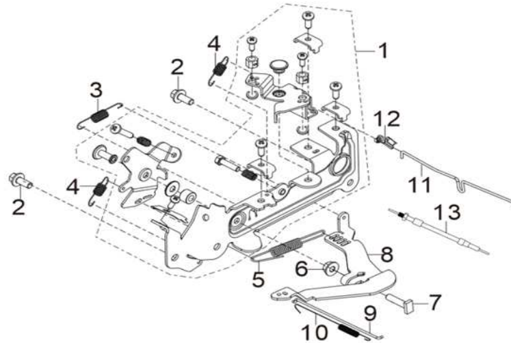
FIG.10 CONTROL ASSY/THROTTLE
