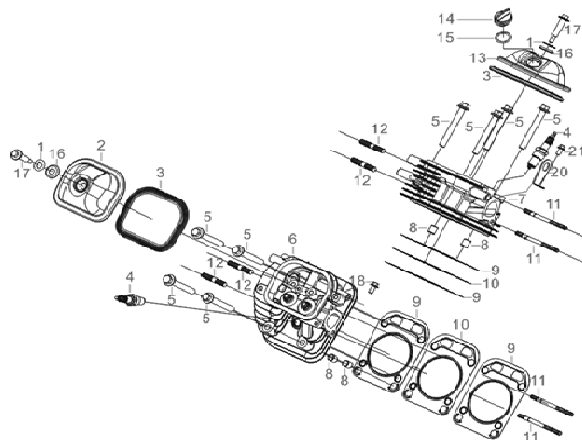
FIG.3 HEAD SUBASSEMBLY, CYLINDER/SPARK PLUG
