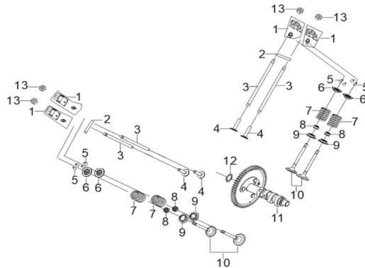
FIG.5 TRAIN, VALVE/CAMSHAFT SUBASSEMBLY
