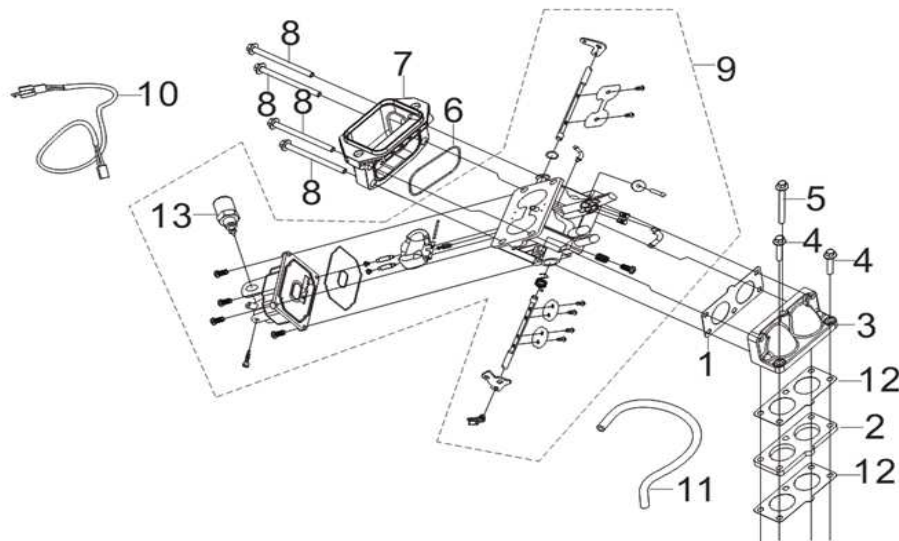
FIG.8 CARBURETOR ASSY
